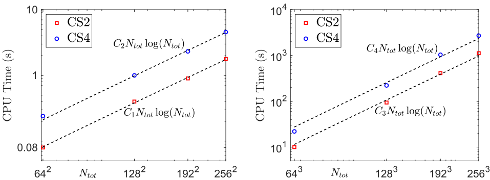
Fig. 1. Log-log plot of CPU time for CS2 and CS4 versus the total grid number N_{\text{tot}} for 2D (left) and 3D (right) cases in Example 3.
