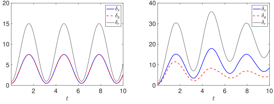
Figure 6: Dynamics of the condensate widths with \gamma=0 (left) and \gamma=3 (right) in Case I of Example 4.5.
