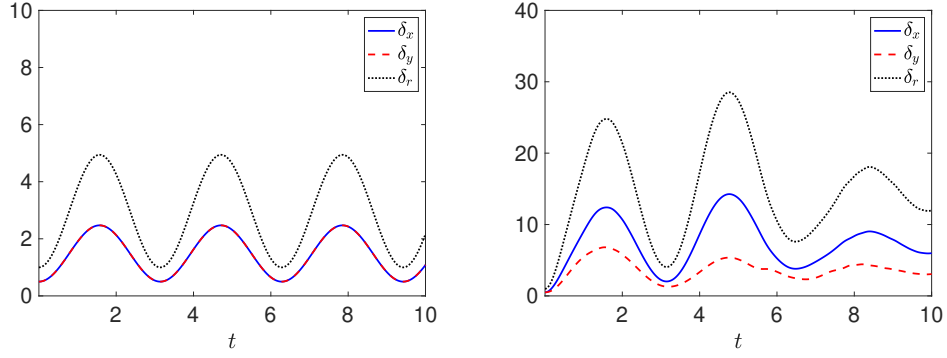
Figure 7: Dynamics of the condensate widths with \gamma=0 (left) and \gamma=3 (right) in Case II of Example 4.5.
