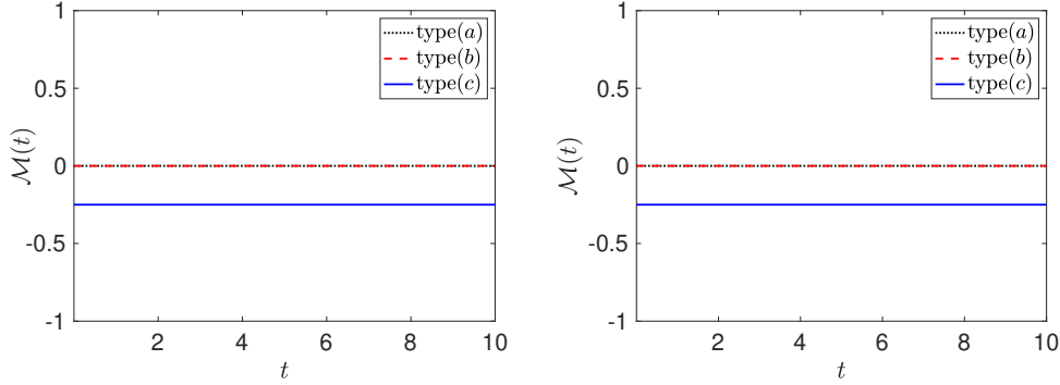
Figure 4: Dynamics of \mathcal{M}(t) with \gamma = 0 for Case I (left) and Case II (right) in Example 4.4.
