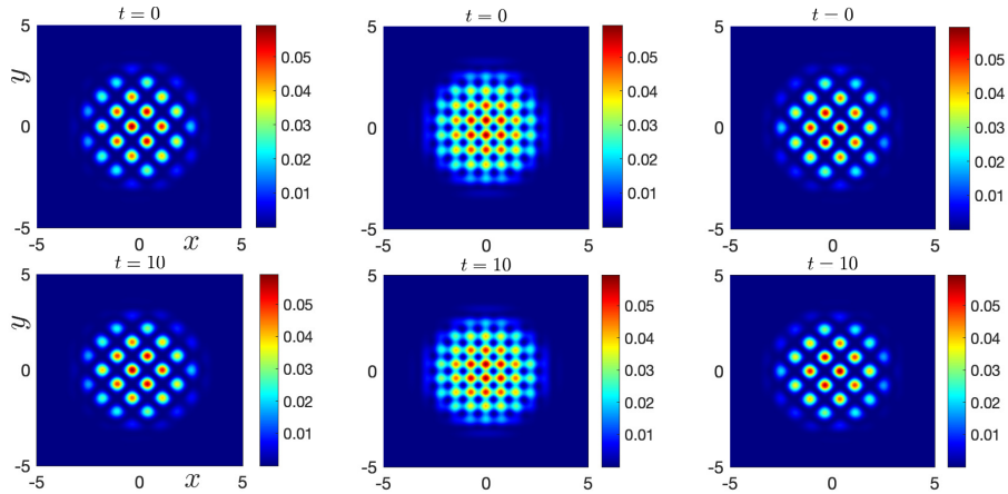
Figure 8: Contour plots of the density |\psi_1|^2 , |\psi_0|^2 and |\psi_{-1}|^2 (from left column to right column) for Case I with the type (e) initial data in Example 4.6.
