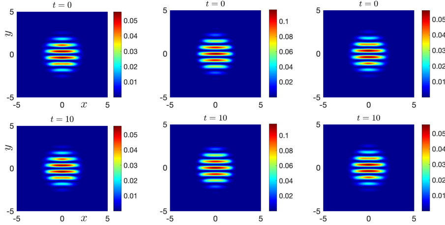
Figure 9: Contour plots of the density |\psi_1|^2 , |\psi_0|^2 and |\psi_{-1}|^2 (from left column to right column) for Case II with the type (e) initial data in Example 4.6.
