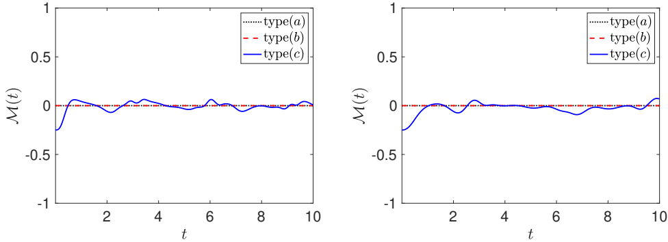
Figure 5: Dynamics of \mathcal{M}(t) with \gamma = 1 for Case I (left) and Case II (right) in Example 4.4.
