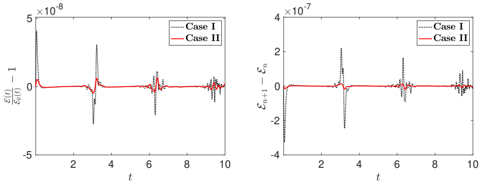
Figure 3: The evolution of \frac{\mathcal{E}(t)}{\mathcal{E}_0(t)} - 1 (left) and \mathcal{E}_{n+1}(t) - \mathcal{E}_n(t) (right) with \gamma = 1 for Case I and Case II in Example 4.3.
