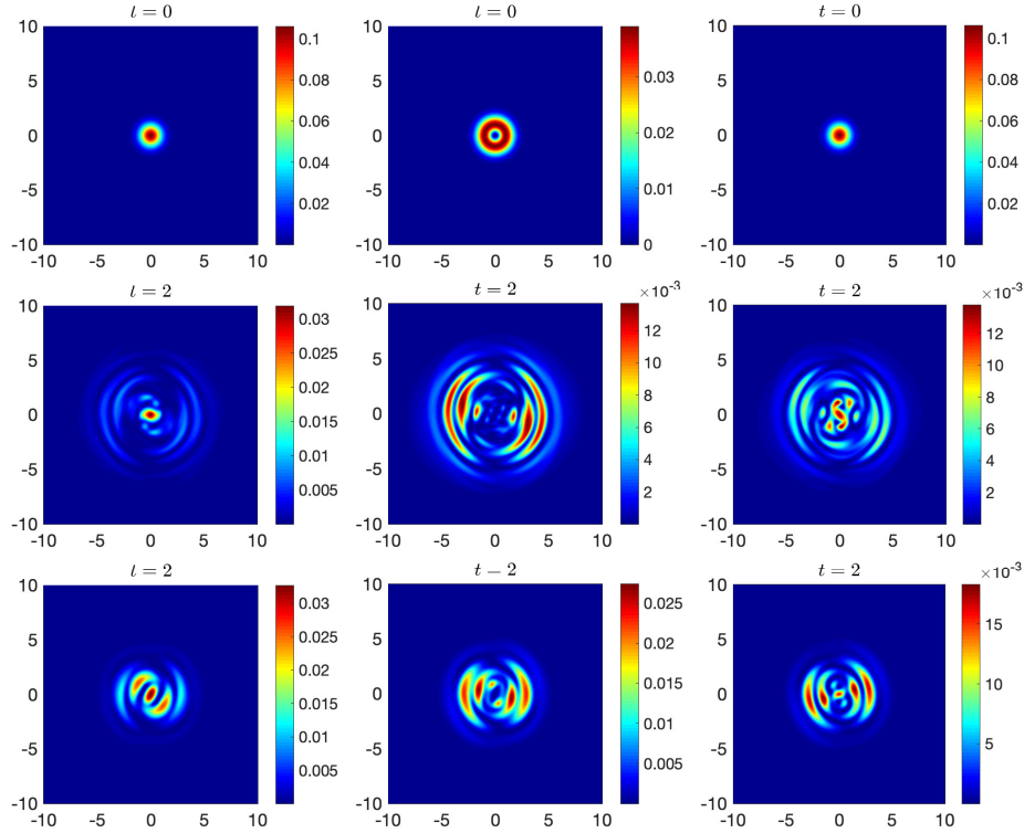
Figure 9: Contour plots of the density |\psi_1|^2 , |\psi_0|^2 and |\psi_{-1}|^2 (from left column to right column) for Case II with the type (e) initial data in Example 4.6.
