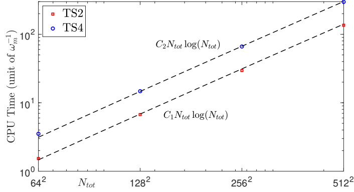
Figure 1: Log-log plot of timing results for TS2 and TS4 versus the total grid number N_{tot} in Example 4.2.
