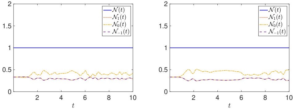
Figure 2: The evolution of total mass \mathcal{N}(t) and component masses \mathcal{N}_\ell(t) ( \ell = 1, 0, -1 ) with \gamma = 1 for Case I (left) and Case II (right) in Example 4.3.
