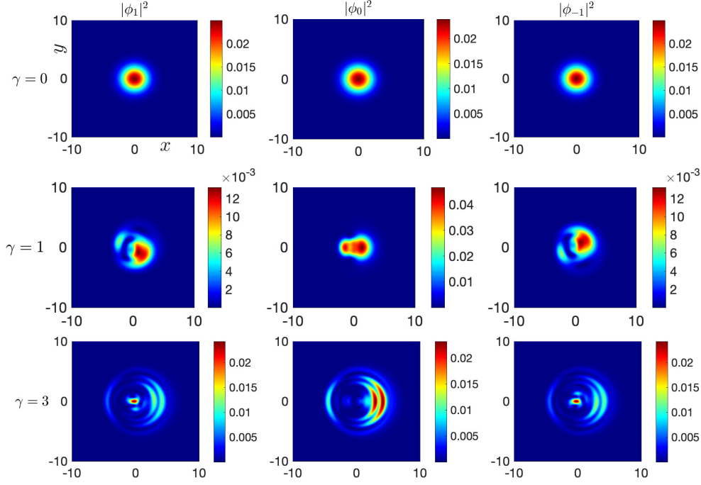
Figure 12: Contour plots of the density |\psi_1|^2 , |\psi_0|^2 and |\psi_{-1}|^2 (from left column to right column) at t=2 in Example 4.7 for Case II with \gamma=0, 1 and 3 (from upper row to bottom row), respectively.
