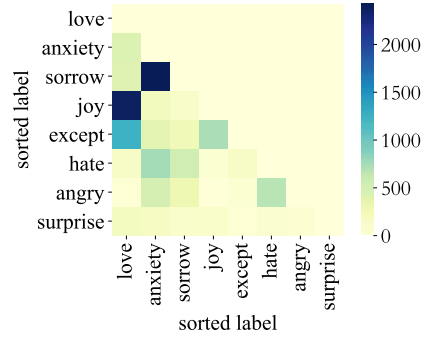
(b) Label co-occurrence of the Ren-CECps dataset.
