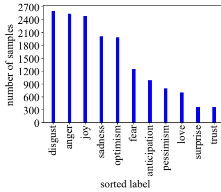
(c) Label distribution of the SemEval18 dataset.
