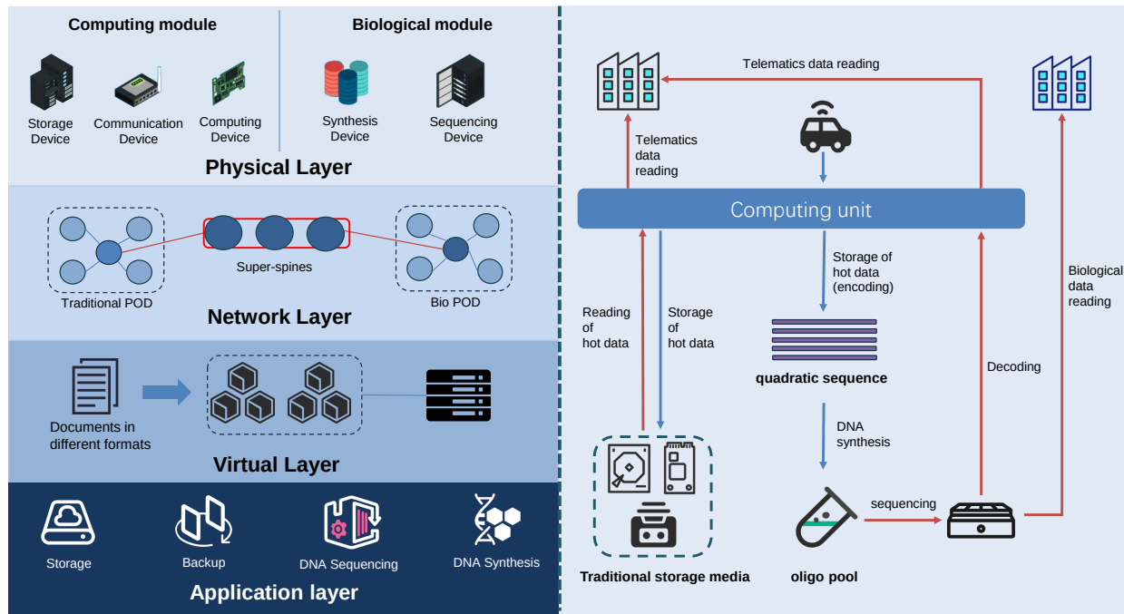
Fig. 3: Data Center Framework Diagram Incorporating DNA Storage
