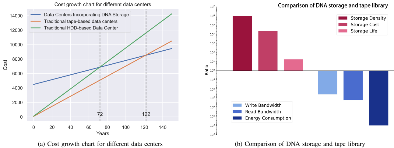
Fig. 4: Effectiveness of data centers incorporating DNA storage vs. traditional data centers. (a) shows the trend of operating costs for storing 1ZB of data under different data centers, where the storage ratio of data centers incorporating DNA storage is 70% DNA storage, 15% HDD storage, and 15% SSD storage, and the storage ratio of storage centers based on tape libraries is 60% tape storage, 25% HDD storage, and 15% SSD storage; and the storage ratio of HDD-based storage centers is 85% HDD and 15% SSD storage. The operating cost per unit time is estimated based on the adjustment of [8]. (b) shows the performance comparison between DNA storage and its main alternative storage medium, the tape library.
