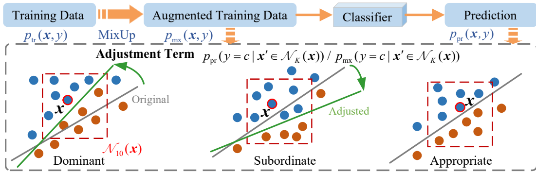
Figure 2: Illustration of Heuristic-CALA. Blue and orange dots represent samples from two classes. The gray and green lines denote the original and adjusted classifiers. The red boxes indicate the ten-nearest neighborhood \mathcal{N}_{10}(\mathbf{x}) . If p_{\text{pr}}(y = y_{\mathbf{x}} | \mathbf{x}' \in \mathcal{N}_K(\mathbf{x})) > (<, =) p_{\text{mx}}(y = y_{\mathbf{x}} | \mathbf{x}' \in \mathcal{N}_K(\mathbf{x})) , then \mathbf{x} is in a dominant (subordinate, appropriate) position in the training set. Our adjustment term will make \mathbf{x} easier (or harder, or leave it unchanged) than before, facilitating better adjusting the classifier.
