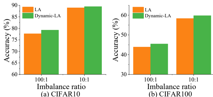
Figure A-3: Top-1 accuracy of LA and Dynamic-LA on CIFAR10-LT (a) and CIFAR100-LT (b) with the imbalance ratios of 10:1 and 100:1.
