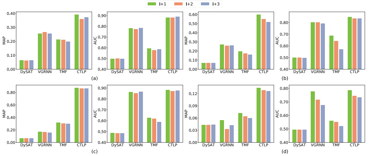
Fig. 4. Multi-step link prediction results in terms of MAP and AUC values of different methods across various real-world networks (a) HS12. (b) ENRON. (c) Cellphone. (d) Ucinmsg.
