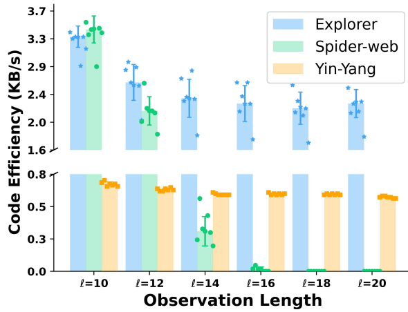
Fig. 6. Comparison between Explorer , SPIDER-WEB and Yin-Yang . (A) The Coding efficiency comparison between Explorer , SPIDER-WEB , and Yin-Yang . The scatter point represents the results of individual experiments, while the histogram heights are constructed from the means of seven experiments. (B) The number of the parameter comparison between Explorer and SPIDER-WEB .
