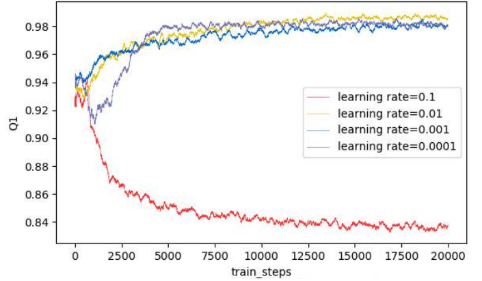
Fig. 6: The impact of the learning rate
