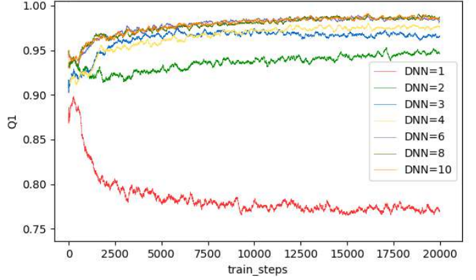
Fig. 5: The impact of the number of DNNs
