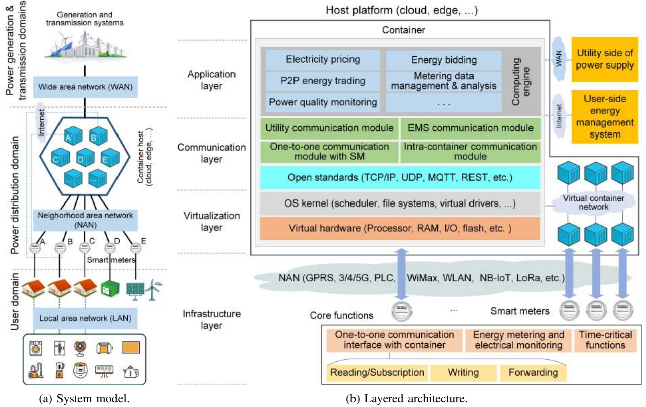
Fig. 2: The container-driven service architecture.
