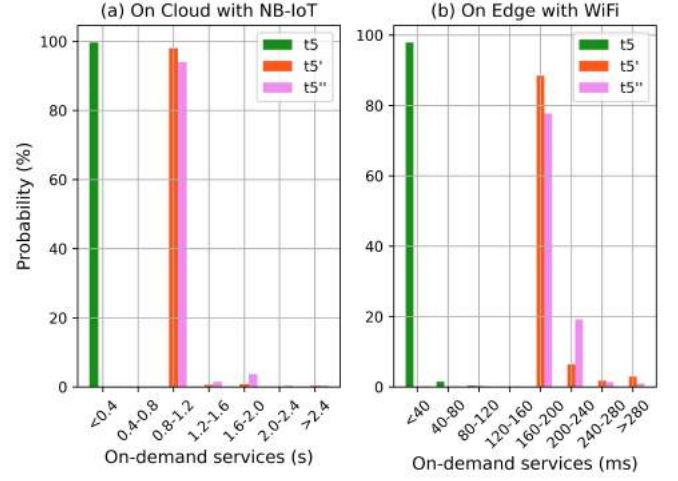
Fig. 12: Communication delays of on-demand services.
