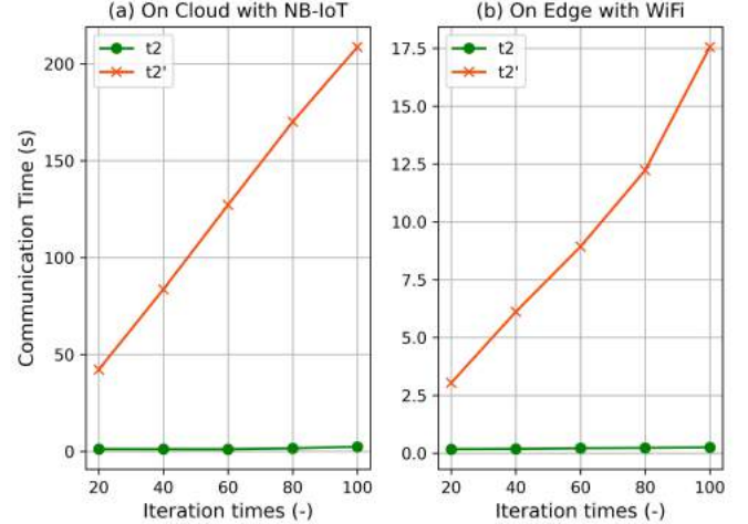
Fig. 9: Communication times of peer-to-peer applications.
