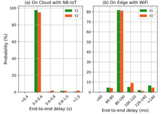
Fig. 8: Statistical probability of end-to-end delays between smart meters and application servers.
