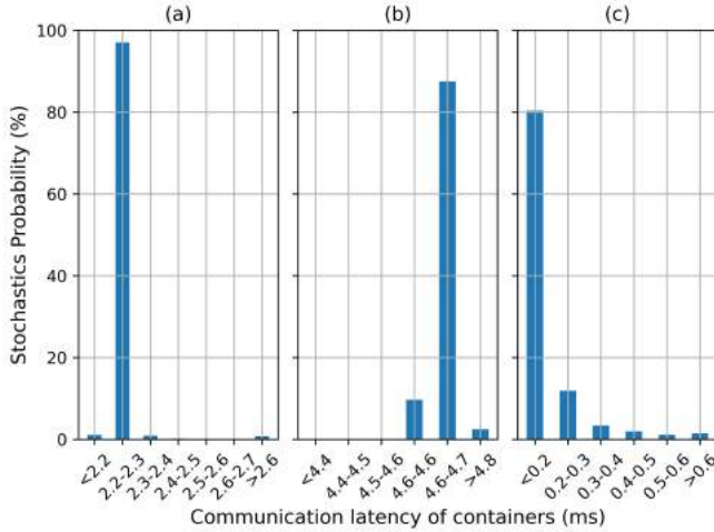
Fig. 11: Communication delays between containers: (a) within the same cloud cluster; (b) in different clusters; and (c) within an edge system.
