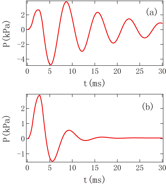
Figure 5. (a) Simulated P(t) with R_2 calculated via equations (4) and (5). (b) Simulated P(t) with R_2 = 5.5 \times 10^6 , which is significantly larger than R_H obtain from equation (4) and (5) for Helmholtz frequency.
