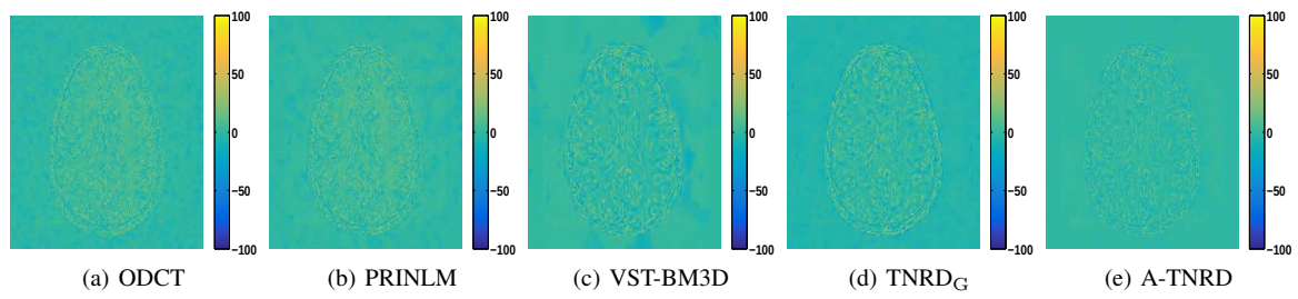
Fig. 14: The difference images between the ground truth and the restoration of ODCT, PRINLM, VST-BM3D, TNRD G , A-TNRD in Fig. 13.
