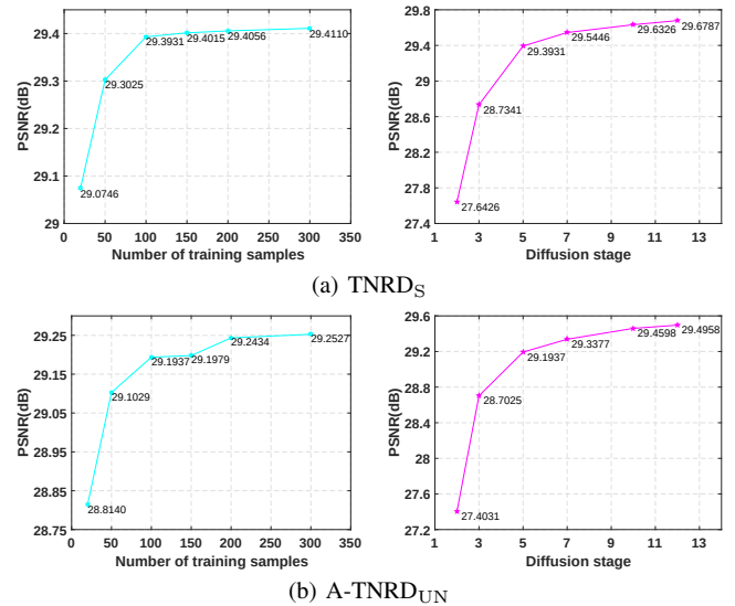
Fig. 4: The influences of the number of training samples and diffusion stages for both TNRD S model and A-TNRD UN model.
