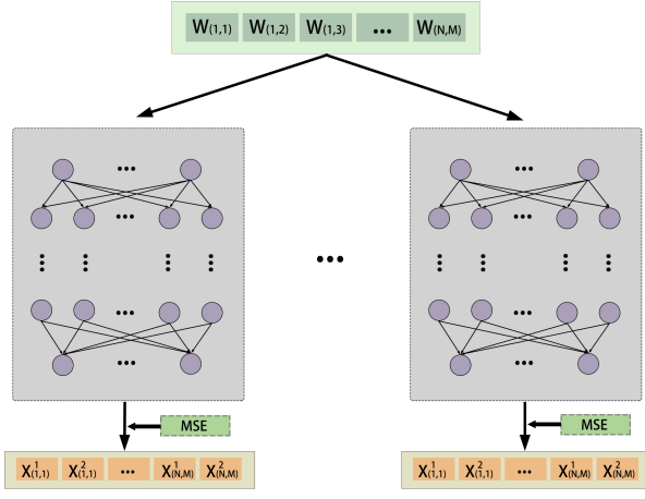
Fig. 3: The process of generating the offloading decisions
