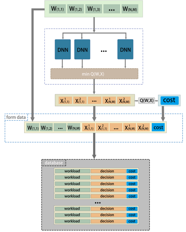
Fig. 2: The procedure of the DDTO algorithm
