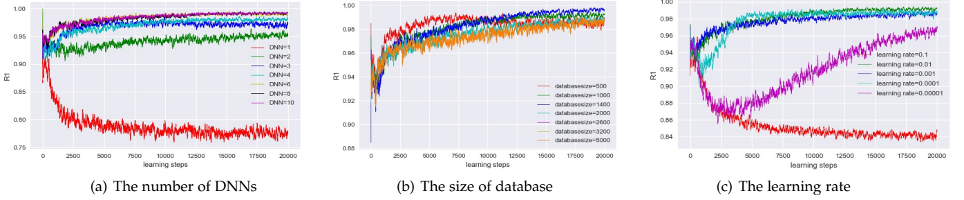
Fig. 4: Impact of the number of DNNs, the size of the database and the learning rate on R_1
