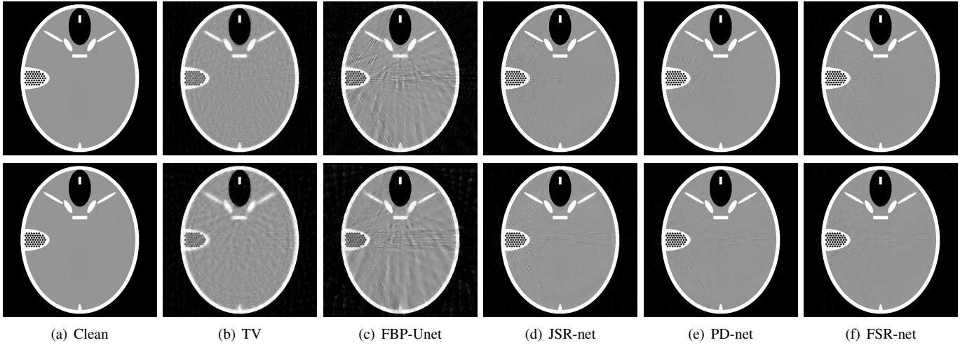
Fig. 5. From row one to row two are reconstruction comparison on the Forbild head phantom with 60 views and 45 views, where the results of the FSR-net is obtained using the SFS system matrix.
