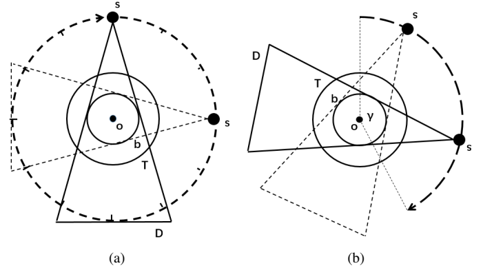
Fig. 1. Sketch map of fan-beam scanning geometry for CT reconstruction: (a) Sparse-view CT Reconstruction; (b) Limited-angle CT Reconstruction. In the figures, s denotes the X-ray source, T denotes the turntable, b denotes the field-of-view, D denotes the detector array, o denotes the rotation center of the X-ray source, and \gamma denotes the rotation angle, which is less than 180^\circ plus the fan-angle for limited-angle CT.
