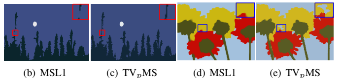
Fig 14. Experiments on multi-phase color image segmentation. The parameters for the MSL1 model are r = 2, 1 , \mu = 100000, 55000 , \lambda = 1.6, 25 and our TV_pMS model are \mu = 200000, 50000 , \lambda = 80, 0.8 .
