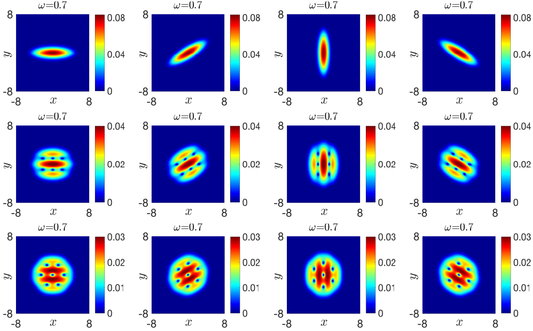
Figure 4: Example 4.4. Contour plot of the density |\phi_g|^2 of the ground states of the 2D rotating dipolar BEC with \lambda = 250, 175, 100 (top to bottom) in Case 1 for \theta = 0, \frac{\pi}{6}, \frac{\pi}{2}, -\frac{\pi}{6} (left to right).
