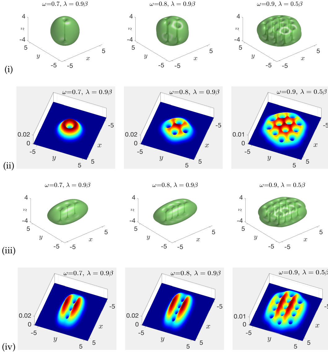
Figure 7: Example 4.6. Isosurface |\phi_g(\mathbf{x})|^2 = 4e-4 ((i) & (iii)) and surface plot of |\phi_g(x, y, z=0)|^2 ((ii) & (iv)) for the six cases (top to bottom then left to right). The CPU cost for these six cases are respectively 5418s, 6845s, 5073s, 4404s, 23408s, 5289s.
