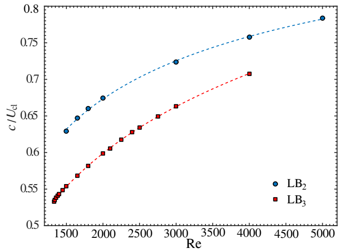
FIG. 5. Reynolds number dependence of the group velocity c with which the localized solutions \text{LB}_2 (circles) and \text{LB}_3 (squares) are advected downstream. The dashed lines are supposed to guide the eye.
