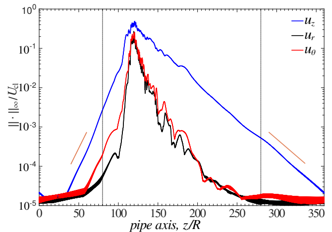
FIG. 9. Axial profiles of infinity norm of the three velocity components for a turbulent puff at Re = 2000 in a pipe of 360R in length. The data are from Song et al. [52]. The orange dashed lines show the spatial decay rates obtained from the LNSE, where m = 1 and m = 0 with c/U_{cl} = 0.5 were used to solve EVP (6) for the upstream and downstream tails, respectively. The dotted vertical lines indicate the locations of the velocity profiles shown in fig. 11.
