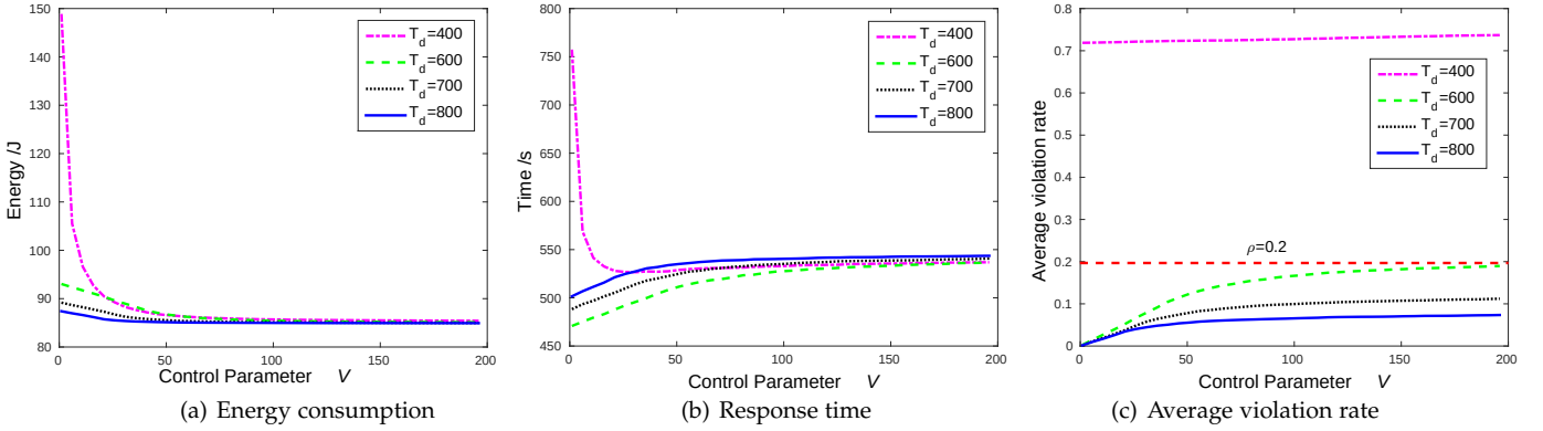
Fig. 12: The impact of V on average the energy consumption, response time and violation rate under different deadlines
