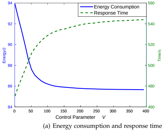
Fig. 10: The impact of V on the average energy consumption, response time and violation rate
