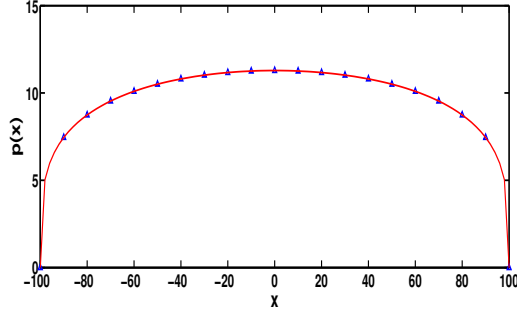
Fig. 4: Behaviors of p(\mathbf{x}) generated by at least 1.5 \times 10^6 trajectories with \beta = 0.5 , n = 1 , r = 100 . The (red) solid line is theoretical result (eq. (44)). The symbols are for the simulation result.
