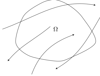
Fig. 6: Sketch map of particles jumping into, or jumping out of, or passing through the domain: \Omega .
