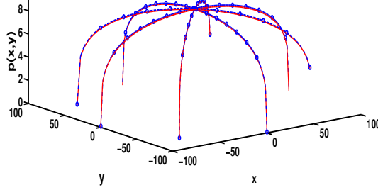
Fig. 5: Behaviors of p(\mathbf{x}) generated by at least 1.5 \times 10^6 trajectories with \beta = 0.5 , n = 2 , r = 100 . The (red) solid line is theoretical result (eq. (44)). The symbols are for the simulation result.
