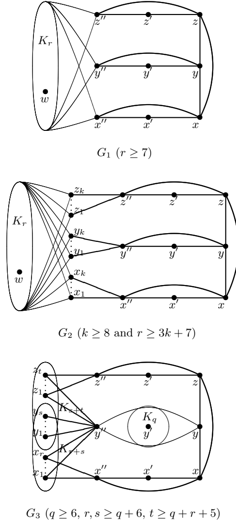
Figure 3 Three classes of claw- \mathcal{o} -heavy non-hamiltonian graphs
