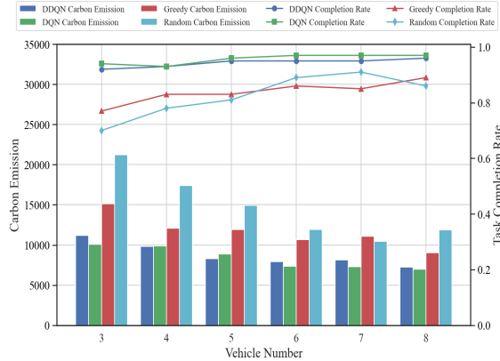
Fig. 4. The carbon emissions and task completion rates of different number of vehicles.
