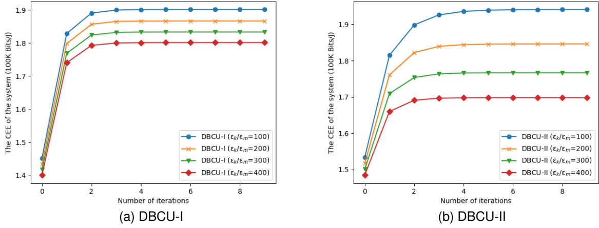
Fig. 6: System CEE under different \varepsilon_k/\varepsilon_m ratios
