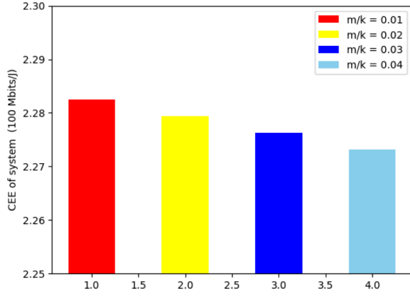
Fig. 9: System CEE under different \varepsilon_m/\varepsilon_k ( m/k )
