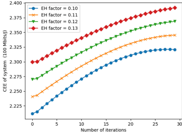
Fig. 10: System CEE under different EH factor \gamma
