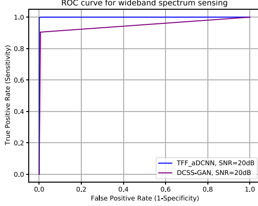
Fig. 11. ROC curve reflecting the classification ability of the model ( SNR = 20\text{dB} , \sigma_1 , m = 20 and N = 6 ).
