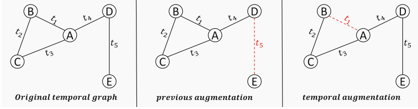
Fig. 1. The toy example illustrates the limitations of the static graph augmentation method when applied to a temporal graph. Specifically, the original temporal network (left) and the resulting loss of temporal information following the application of static graph augmentation (middle) are demonstrated. To address this issue, we propose a novel approach for augmenting temporal graphs by incorporating both topological and temporal information. This approach allows us to eliminate redundant information while preserving vital temporal information (right).
