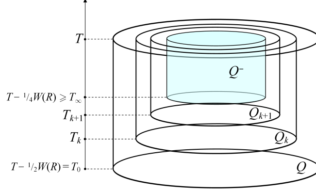
FIGURE 4. Cylinders Q, Q^-, Q_k
