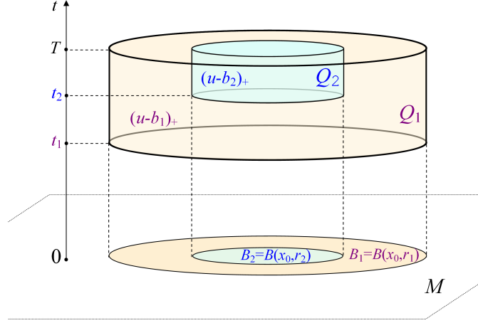
FIGURE 3. Functions (u - b_i)_+ in cylinders Q_i
