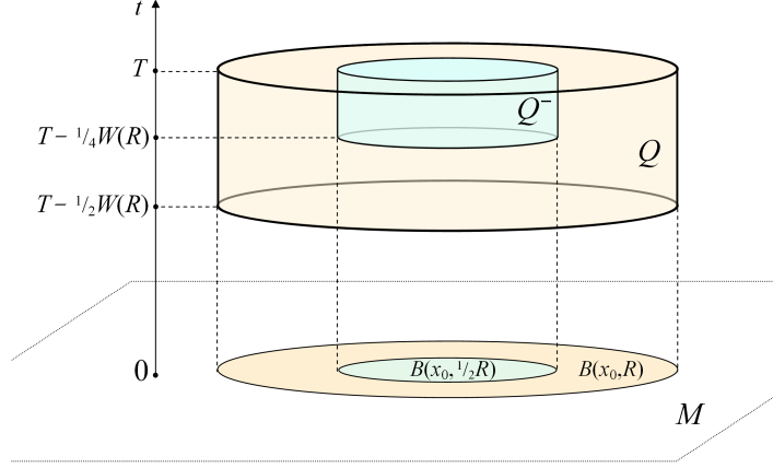
FIGURE 2. Cylinders Q^- and Q
