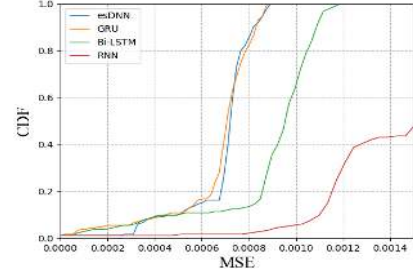
(b) CDF of MSE with Google Trace
