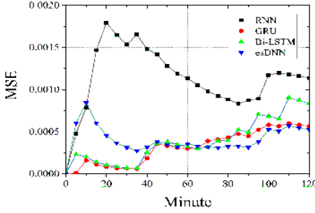
Fig. 10. Prediction accuracy (MSE) of four different RNN methods based on the Google dataset
