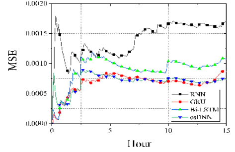
Fig. 10. Prediction accuracy (MSE) of four different RNN methods based on the Google dataset
