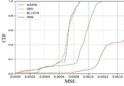
(a) CDF of MSE with Alibaba Trace
