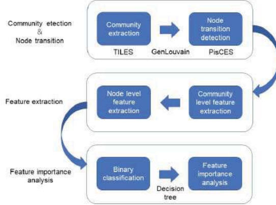
Figure 2: Framework schematic
