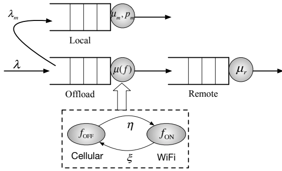
Fig. 3. The partial offloading model
