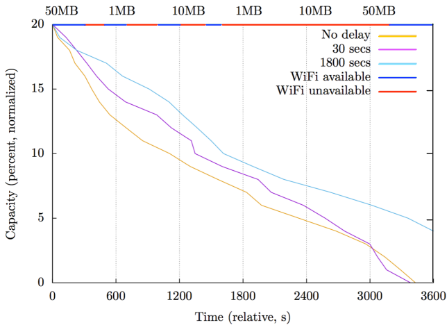
Fig. 16. Capacity discharge over time for different executions
