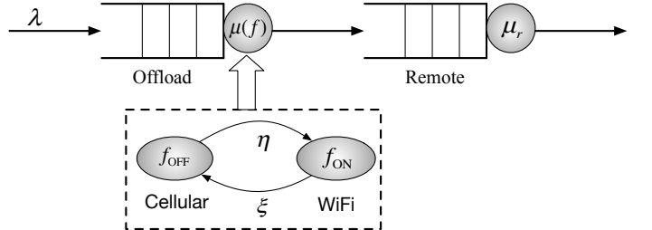
Fig. 5. The non-delayed offloading model
