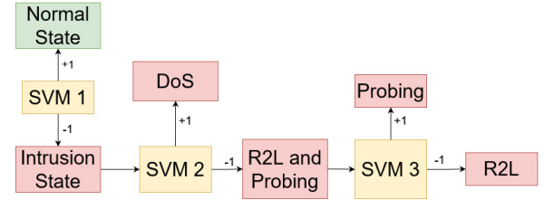
Fig. 4: Intrusion detection system using Multiclass SVM Approach
