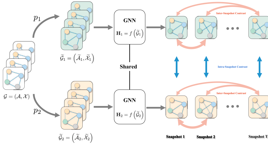
Fig. 2. An overview of our proposed DNCL model. We first create two dynamic network views by augmenting the network structure and node attributes. Then, both views are input into a shared Graph Neural Network (GNN) encoder, which learns representations of the nodes. The model is trained using contrastive objectives, including the inter-snapshot contrast of node representations within the same views of different snapshots (red arrows) and the intra-snapshot contrast of node representations between two views of the same snapshots (blue arrows).
