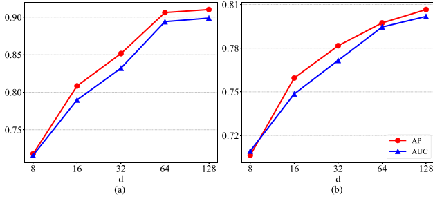
Fig. 5. Influence of embedding dimension for AP and AUC scores on two datasets. (a) Enron. (b) Cell.
