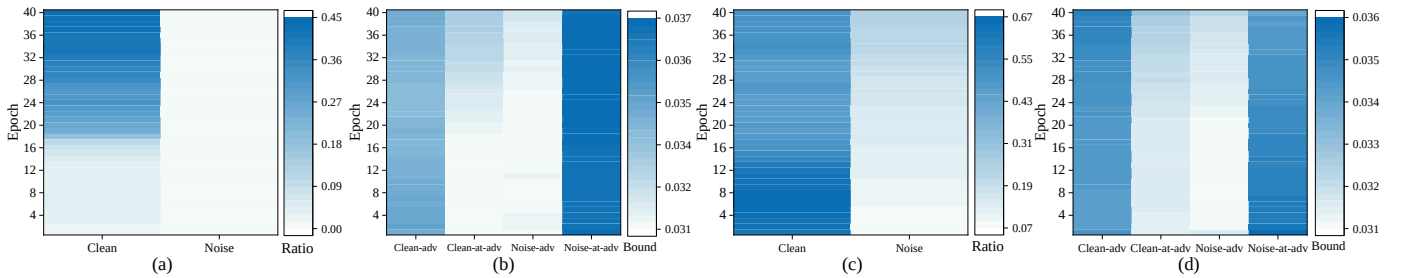
Fig. 10. (a): Ratio of adversaries for noisy and clean samples on CIFAR10 with 20% uniform noise during training. (b): Average adversarial and anti-adversarial perturbation bounds for clean and noisy samples on CIFAR10 with 20% uniform noise during training. (c): Ratio of adversaries for noisy and clean samples on CIFAR10 with 40% pair-flip noise during training. (d): Average adversarial and anti-adversarial perturbation bounds for clean and noisy samples on CIFAR10 with 40% pair-flip noise during training.
