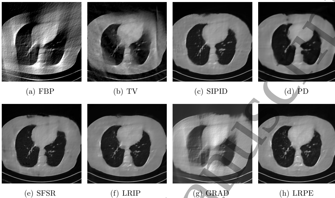
Figure 10. Limited-angle reconstruction experiment of the AAPM phantom dataset with 90^\circ scanning angular range and 5% Gaussian noises.
