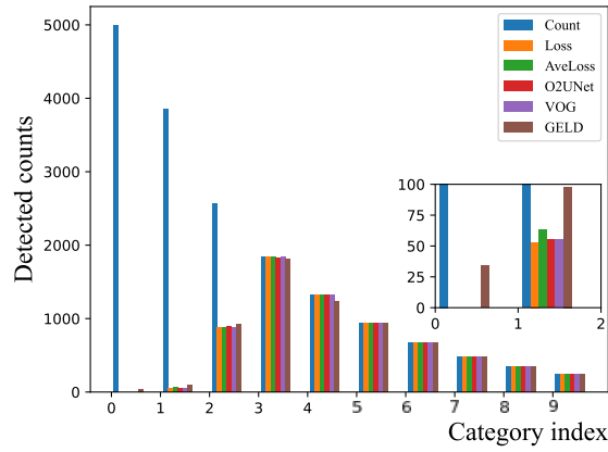
Fig. 15. Histogram of CIFAR10-LT top-40% detected hard samples.
