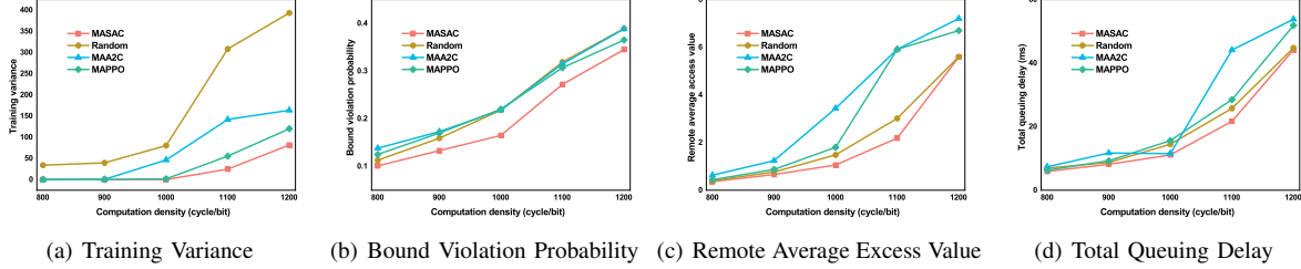
Fig. 8: TV, BVP, RAEV and TQD over time slots with different computation density
