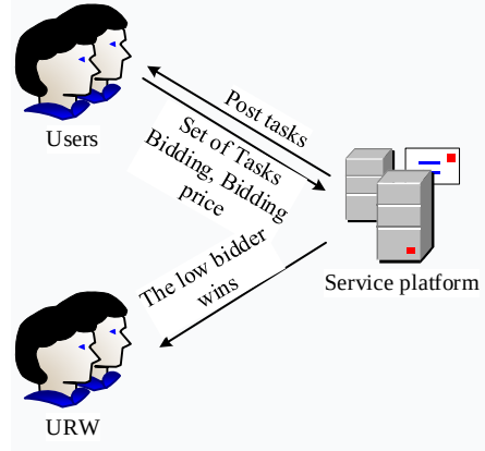
Fig. 1. Reverse auction
