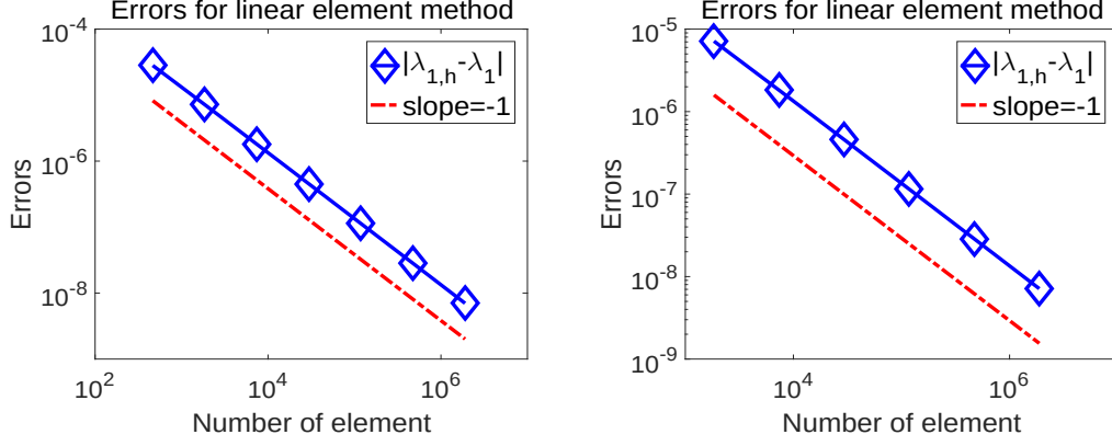
Figure 2: The errors of the multilevel iteration algorithm for the first eigenvalue \lambda_1 on the unit square. (The left subfigure is for the coarse initial mesh in Figure 1 and the right one for the fine initial mesh in Figure 1)
