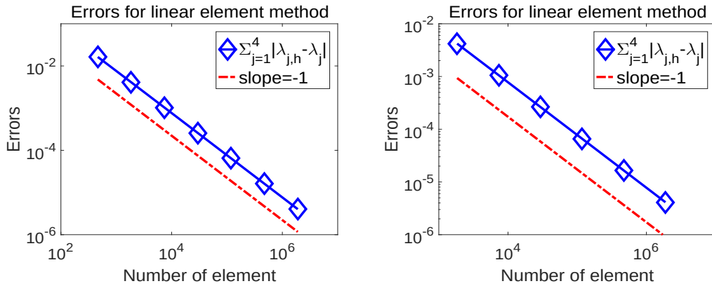
Figure 3: The errors of the multilevel iteration algorithm for the first four eigenvalues on the unit square (The left subfigure is for the coarse initial mesh in Figure 1 and the right one for the fine initial mesh in Figure 1)
