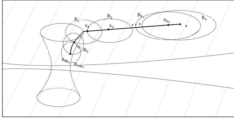
Figure 1: The chosen points and balls along the geodesic.
