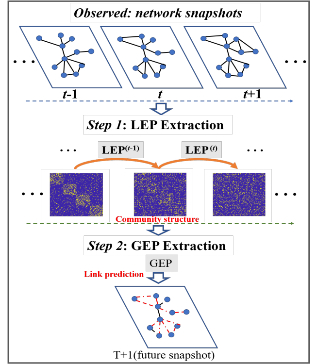
FIGURE 2: Illustration of the proposed ONMF-EEP.
