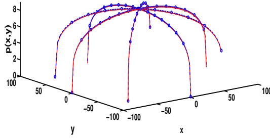
Fig. 5: Behaviors of p(\mathbf{x}) generated by at least 1.5 \times 10^6 trajectories with \beta = 0.5 , n = 2 , r = 100 . The (red) solid line is theoretical result (eq. (44)). The symbols are for the simulation result.
