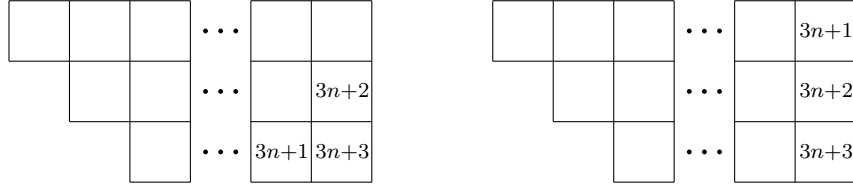
Figure 3.2: The two cases when T(2, n + 2) = 3n + 2
