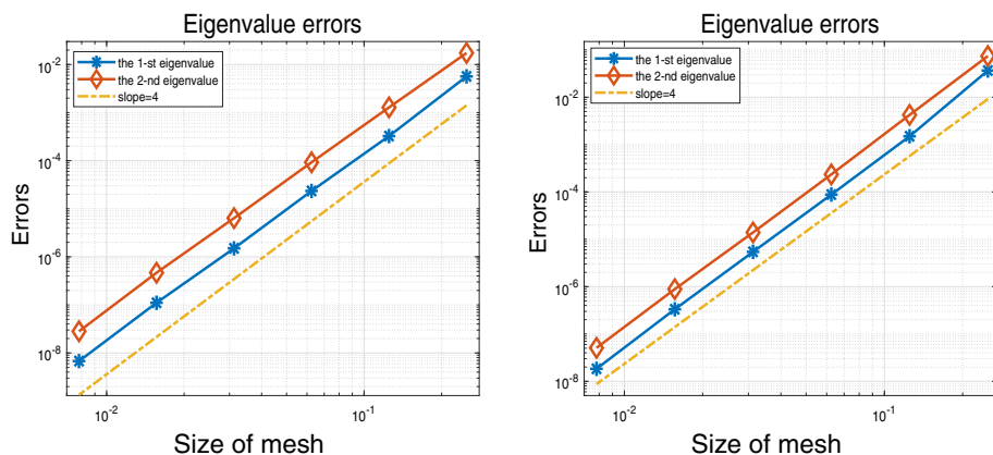
Fig. 8 The errors of the first two eigenvalues by 1st FE group (5.1) (left) and 2nd FE group (5.2) (right) on unit square with k = 1
