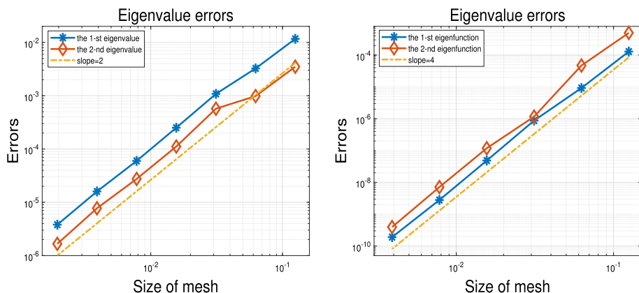
Fig. 2 The errors of the first two eigenvalues with k = 0 (left) and k = 1 (right) on unit square for the initial mesh in Fig. 1
