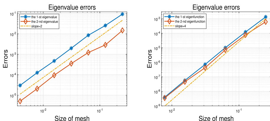
Fig. 4 The errors of the first two eigenvalues with k = 0 (left) and k = 1 (right) on regular hexagon for the initial mesh in Fig. 3
