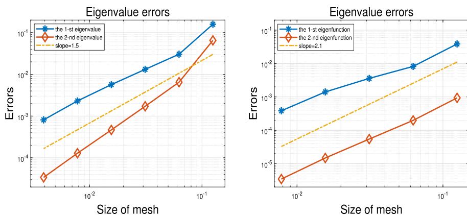
Fig. 6 The errors of the first two eigenvalues with k = 0 (left) and k = 1 (right) on L-shape domain for the initial mesh in Fig. 5
