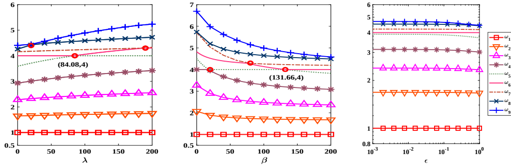
Figure 3: Example 4.5. Eigenvalues \omega_\ell , \gamma_x = 1 , \gamma_y = 4 , \mathbf{n} = (1, 0, 0) . Left: \beta = 200 , \epsilon = 1/\sqrt{60} (Case 1). Middle: \lambda = 40 , \epsilon = 1/\sqrt{120} (Case 2). Right: \beta = 250 , \lambda = 100 (Case 3).
