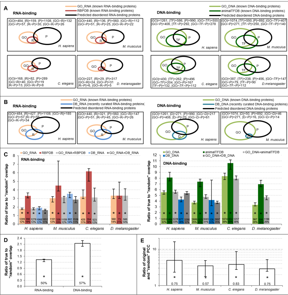
Figure 3. Evaluation of predictions of the disordered RNA-, DNA- and protein-binding in the H. sapiens , M. musculus , C. elegans and D. melanogaster genomes. (A) Venn diagrams of the overlap between the disordered RNA-binding (DNA-binding) proteins predicted by DisoRDPbind and the known binding proteins collected from the GO.RNA (GO.DNA) and RBPDB (animalTFDB) data sets, respectively. (B) Venn diagrams of the overlap between the disordered RNA-binding (DNA-binding) proteins predicted by DisoRDPbind and the known binding proteins collected from the GO.RNA (GO.DNA) and from recently curated RNA-binding (DNA-binding) protein data set DB.RNA (DB.DNA), respectively. The area of the rectangles corresponds to 40% of size of a given proteome; The counts of proteins in a given data set and intersections of the data sets are given inside the corresponding rectangles; (C) Median ratio between the actual overlap between the RNA-binding (DNA-binding) proteins predicted by DisoRDPbind and proteins annotated in the GO.RNA, RBPDB and DB.RNA (GO.DNA, animalTFDB and DB.DNA), and the overlap of the proteins from these databases with a randomly chosen set of proteins. The median ratio is over 10 repetitions with half of the data; error bars are 30% and 70% centiles; the number of chains in a given database and percentage of overlap with the predictions of DisoRDPbind are given inside the bars; * means that the difference between the two values of overlap is statistically significant at P -value < 0.0005 . (D) Median ratio (over 10 repetitions with half of the data; error bars are 30% and 70% centiles) between the actual overlap between the cellular localizations of novel putative RNA (DNA) binders and the localizations that are significantly associated with the proteins known to bind RNA from GO.RNA, RBPDB and DB.RNA (known to bind DNA from GO.DNA, animalTFDB and DB.DNA), and the overlap in cellular localizations of the proteins from these databases with a randomly chosen set of proteins. This analysis was done in M. musculus since annotation of localizations in other genomes were not sufficiently complete. The percentage of the overlap with the predictions of DisoRDPbind is given inside the bars; * denotes that the difference between the two values of overlap is statistically significant at P -value < 0.05 . (E) Relation between the promiscuity of proteins in PPI networks collected from mentha and the number of the disordered protein-binding regions predicted with DisoRDPbind. The relation was quantified with Pearson correlation coefficient (PCC) that is show inside the bars. Bars shows median ratio (over 10 repetitions with half of data; error bars are 30% and 70% centiles) in logarithmic scale between these PCC values and the 'random PCC' where the promiscuity values were shuffled; * denotes that the difference between the two values of PCC is statistically significant at P -value < 0.05 .
