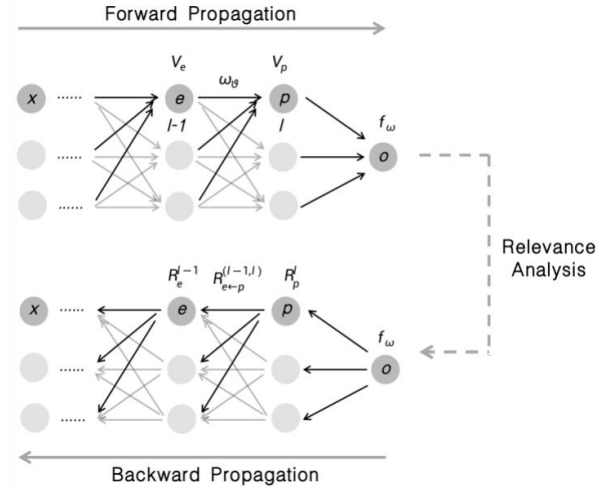
Fig. 3: The process of layer-wise relevance analysis method of Deep-DPGI based on back propagation algorithm
