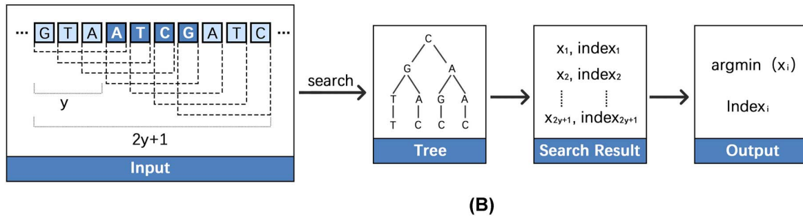
Figure 3. Node drift diagram. (A) indicates horizontal drift, for a specific sequence ACCG , which has no matching node in the second layer of the tree, for which we can candidate drift to T or G nodes, but we require that the subsequent two consecutive nodes of the drift node are not allowed to drift again, so the branches ATTA and AGCT are not satisfied, for which the final match to the branch is AGCG , with a drift count of 1. (B) indicates the longitudinal drift, where the longitudinal drift y value is 3. When selecting intervals for tree retrieval, the interval with the most y bits of displacement before and after the original interval is allowed to be selected. After subjecting a total of 2y + 1 intervals to tree retrieval, the algorithm will output the smallest lateral drift value and the corresponding index.
