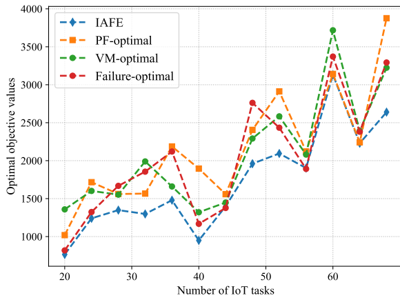
Fig. 4. The performance comparison of four approaches
