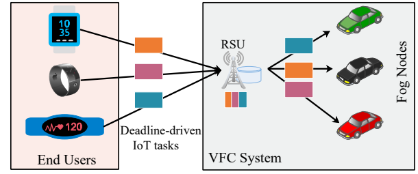
Fig. 1. Failure-aware VFC architecture for deadline-driven IoT tasks
