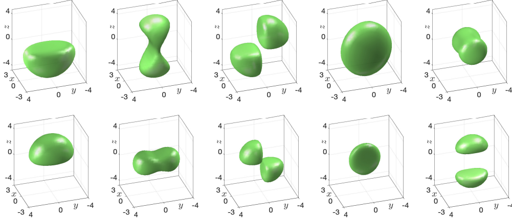
FIG. 4. Isosurface plots of the Bogoliubov amplitude of u_\ell = 10^{-3} (upper), v_\ell = 10^{-3} (lower) (left to right: \ell = 1, \dots, 5 ) for Case II in Example 5.
