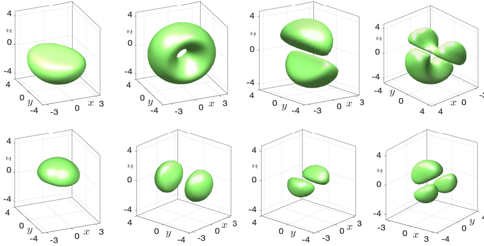
FIG. 3. Isosurface plots of the Bogoliubov amplitude of \mathbf{u}_\ell = 10^{-3} (upper), \mathbf{v}_\ell = 10^{-3} (lower) (left to right: \ell = 1, \dots, 4 ) for Case I in Example 5.
