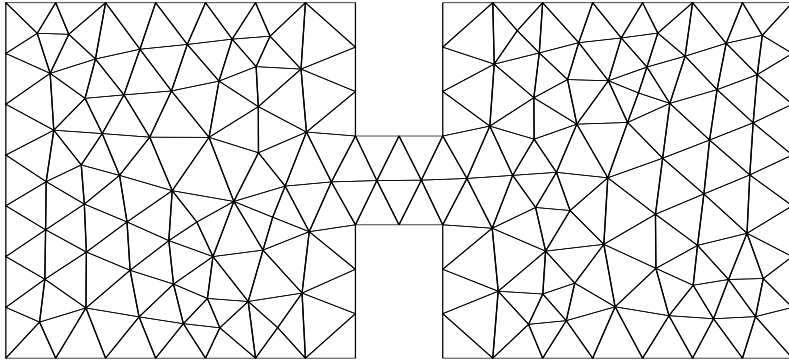
Figure 3: The initial/coarsest mesh for Example 2
