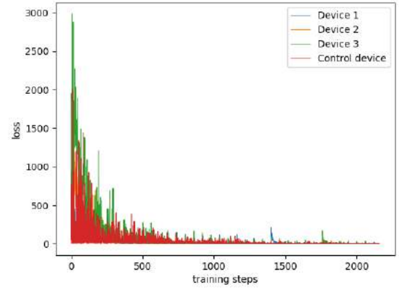
Figure 5: The convergence performance under different devices
