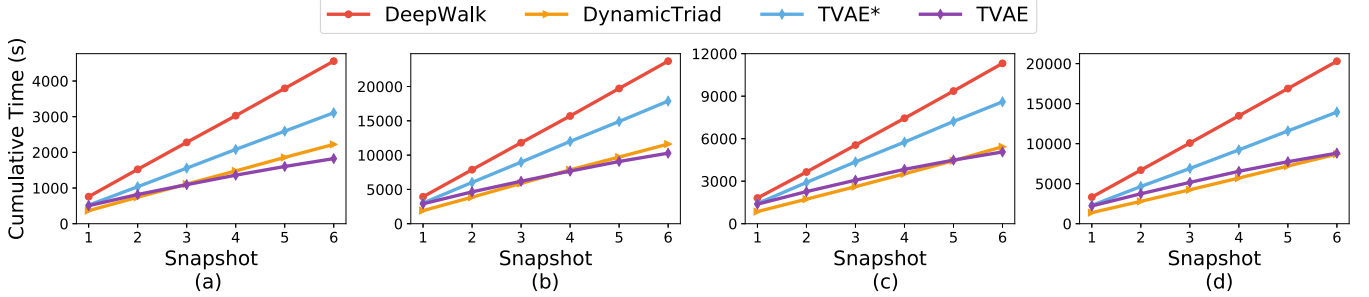
Fig. 5. Cumulative time cost of different algorithms. We compute the time cost of Deepwalk, DynamicTriad, and TVAE on different data sets. We choose six continuous snapshots for evaluation and obtain the cumulative time cost curves of different algorithms. TVAE* is our proposed model without applying the parameter inheritance mechanism. (a) SBM (1000). (b) SBM (5000). (c) Hep-th. (d) AS.
