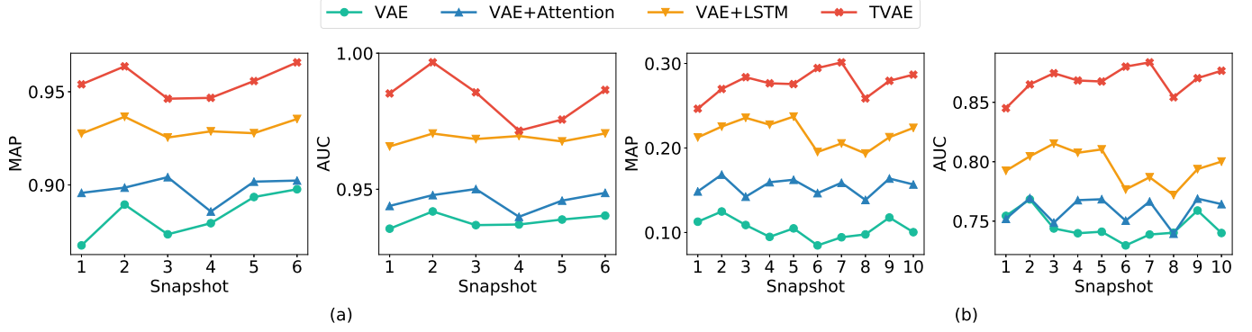
Fig. 4. Ablation experiments of our TVAE and its parts VAE, VAE+attention on two different networks (a) SBM(1000). (b) BC-OTC.
